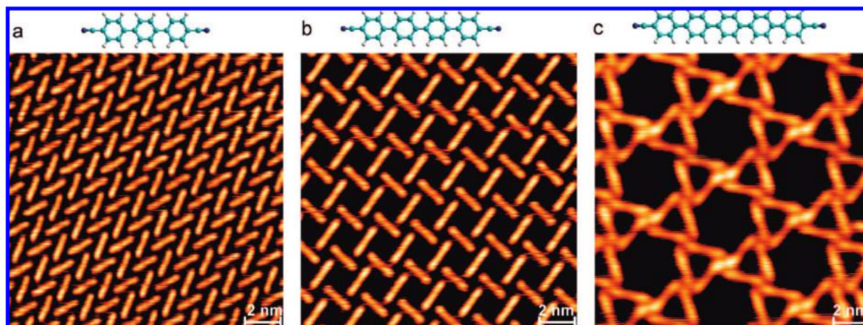
Figure 1. Steering network complexity with the extension of the molecules self-assembled on the Ag(111) surface. (a) Densely packed chevron layer formed by the NC-Ph 3 -CN species. (b) NC-Ph 4 -CN molecules assemble in an open rhombic network. (c) Kagomé lattice formed by NC-Ph 5 -CN molecules, comprising four-fold nodes and quasi-hexagonal and trigonal cavities. These images and the following were taken at surfaces covered with the molecular networks in the submonolayer regime and were recorded at 10 K. Structure models of molecular building blocks are depicted above the STM images. Their respective lengths are 1.66, 2.09, and 2.53 nm (light blue, C; dark blue, N; gray, H).
